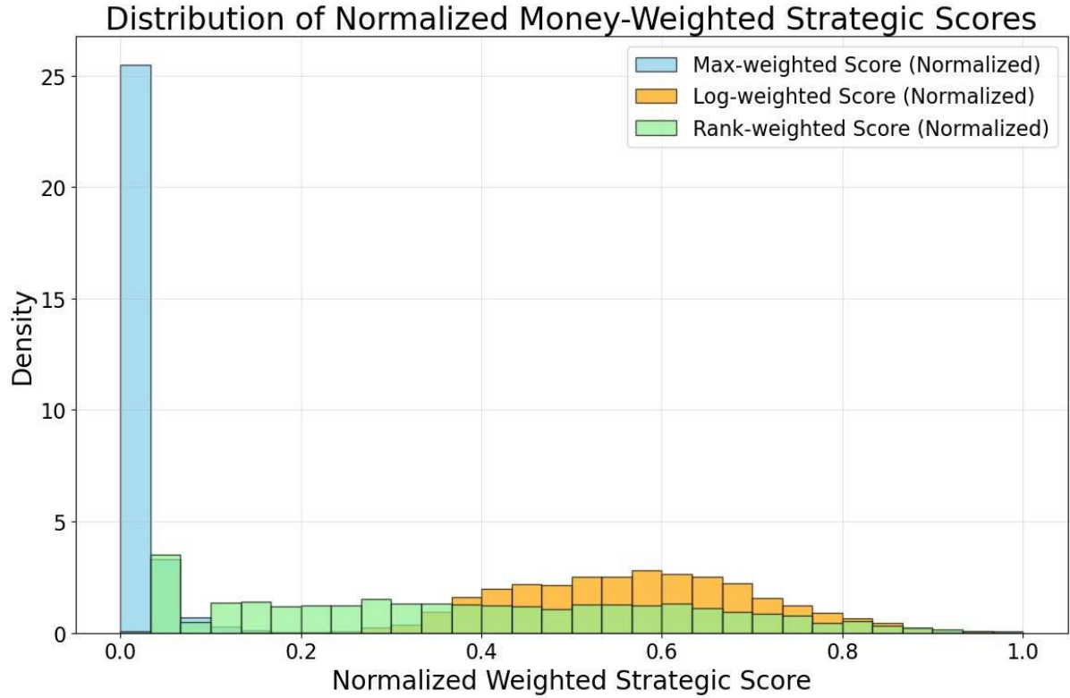
Figure 11: The figure displays the impact of different money-weighting techniques on the distribution of normalized strategic alignment scores, highlighting how weighting choice affects the score’s aggregation.
