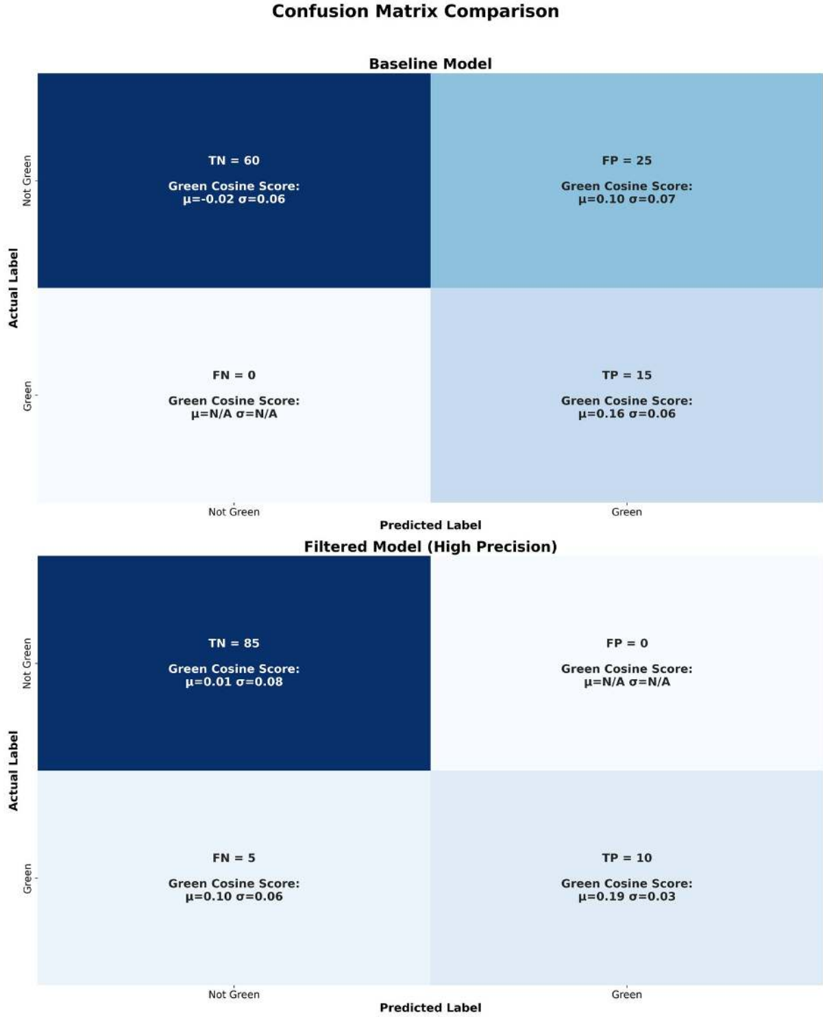
Figure 8: Confusion matrices comparing the Baseline and Filtered (High Precision) models, with cosine similarity scores for 'Green' predictions. The Baseline model achieves full recall but at the cost of many false positives, reflected in lower cosine similarity for incorrect predictions. The Filtered model eliminates false positives, improving precision and alignment with the embedding space, as confirmed by significantly higher cosine scores for retained true positives ( p = 0.0007 )
